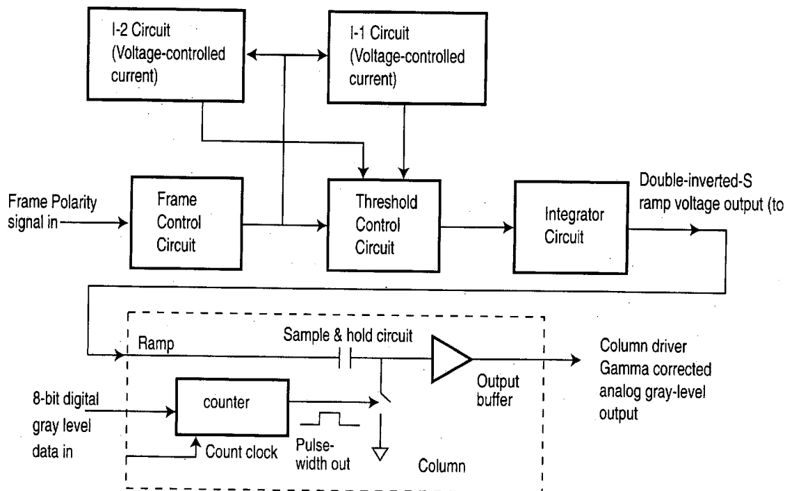
Block Diagram of Non-linear Ramp Generator for Gamma Correction of EL Panels
